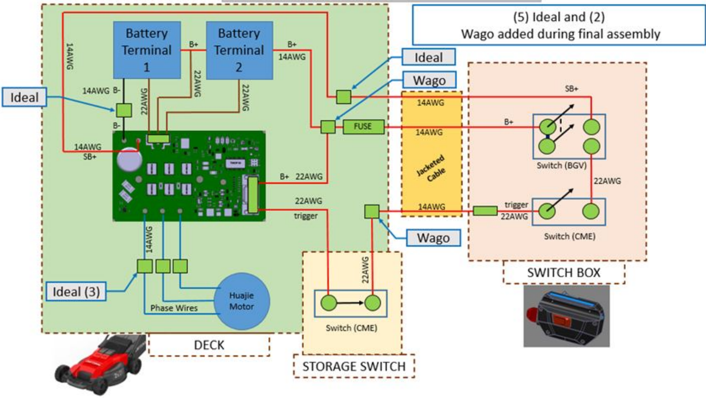
Craftsman 2x20V Mower: EE Block Diagram Rev 01
